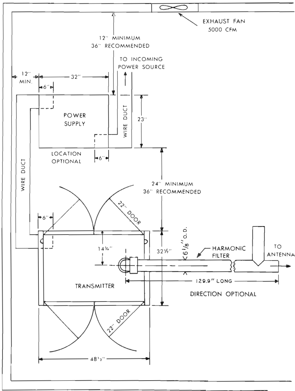
FIG. 7. Floor plan layout for BTF-20E transmitter.
