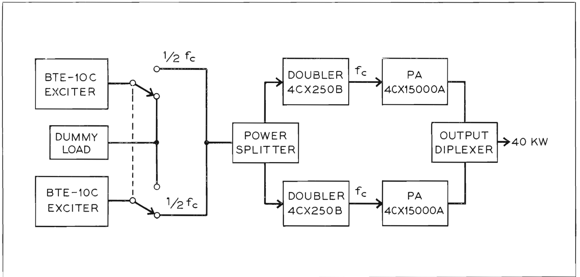
FIG. 2. Block diagram of 40 kW transmitter showing power splitter, output combiner (diplexer), and switch for selecting either of two operating exciters.
