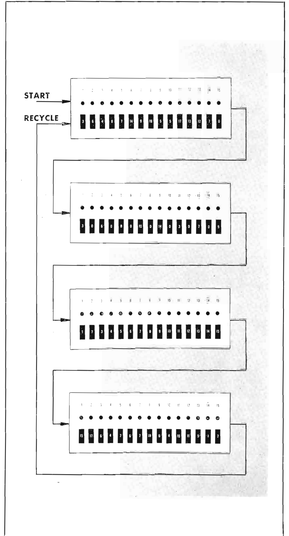
FIG. 8. Four BCA-15 units cascaded to provide a 60-event system.
