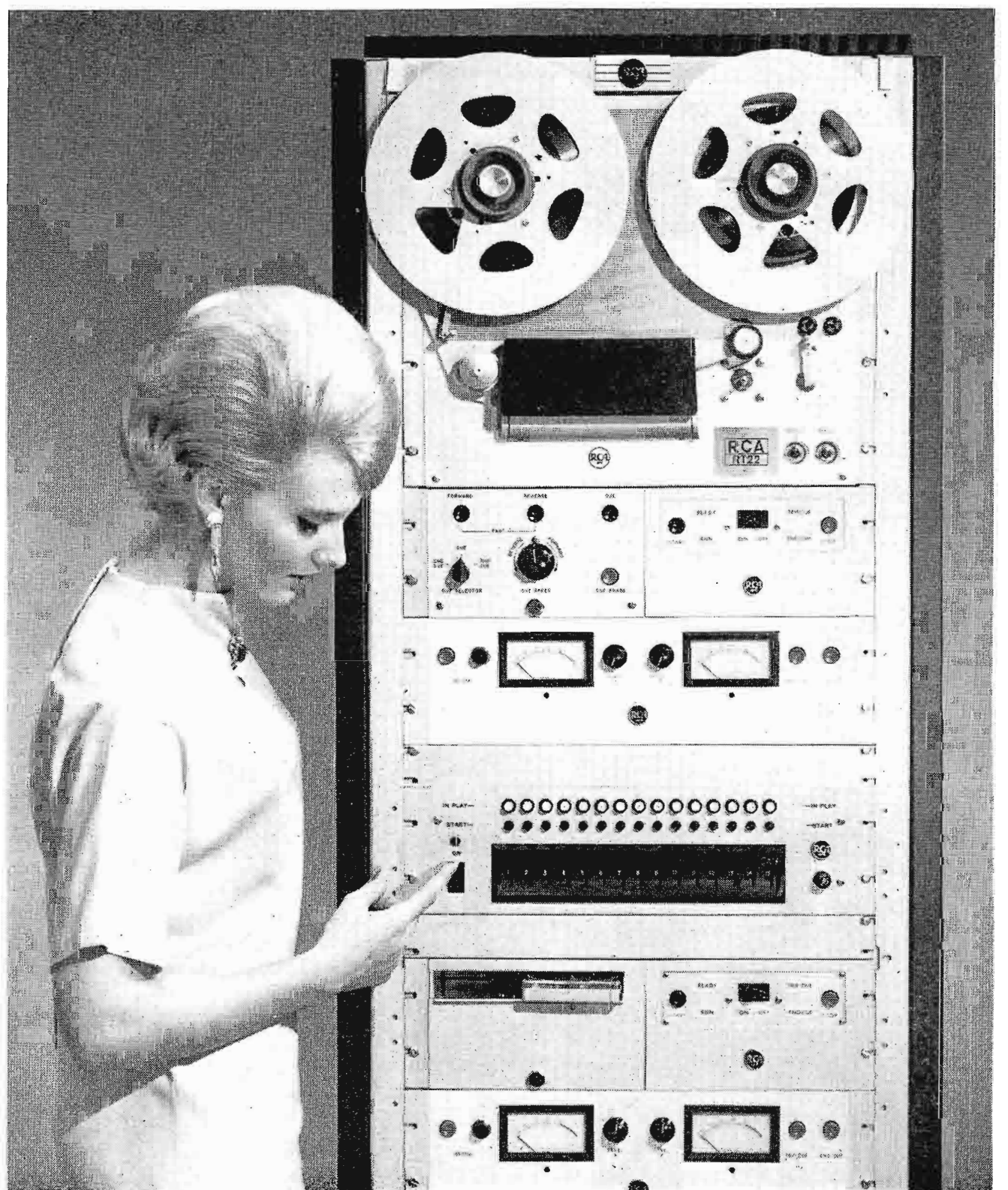
FIG. 12. BCA-15 shown with RT-22 reel recorder (top) and RT-8 cartridge recorder (bottom).
