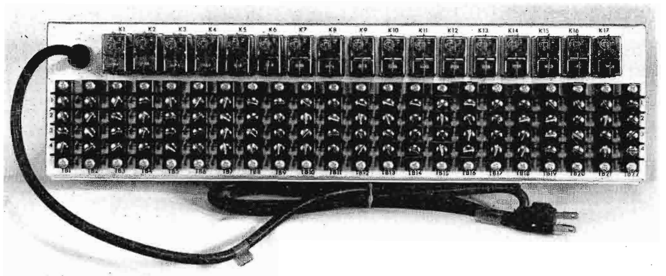
FIG. 11. Rear view of BCA-15 showing switching and program line interconnection terminals.
