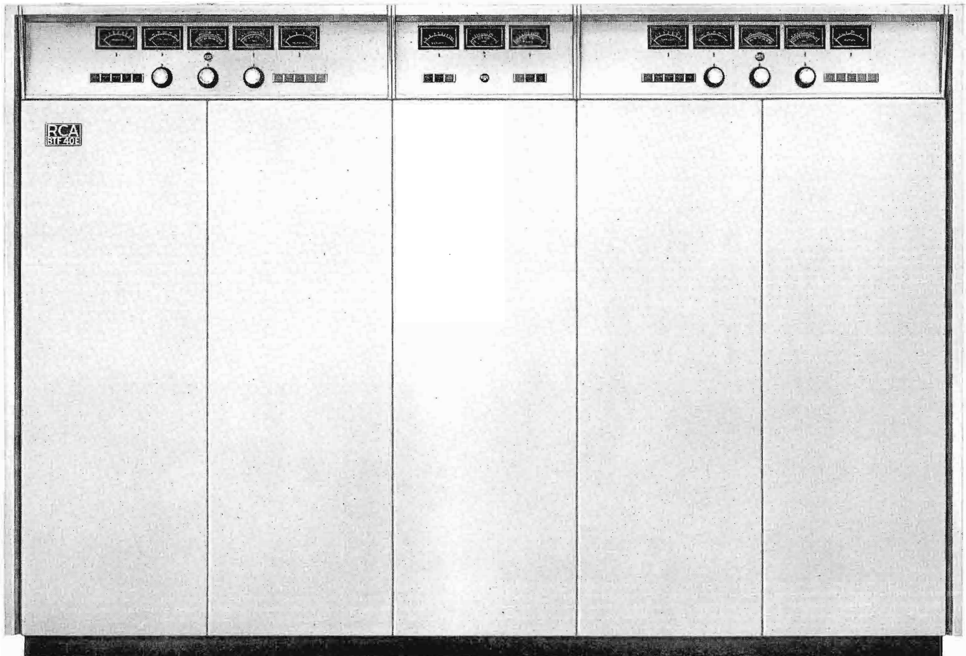
FIG. 1. Type BTF-40E FM transmitter offers unexcelled reliability by combining the outputs of two 20 kW units. Combining equipment is housed in center cabinet.
