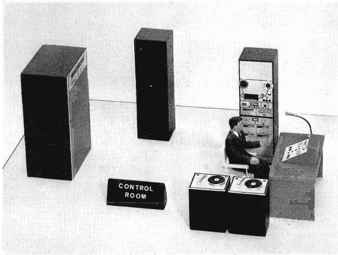
FIG. 3. Plan "A" control room with transmitter, cartridge and reel tape recorders, audio console and transcription turntables.
