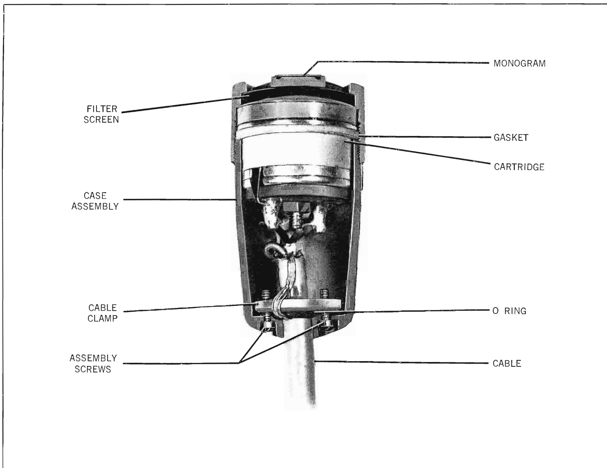
FIG. 5. Cross-section view showing details of BK-12A construction.
