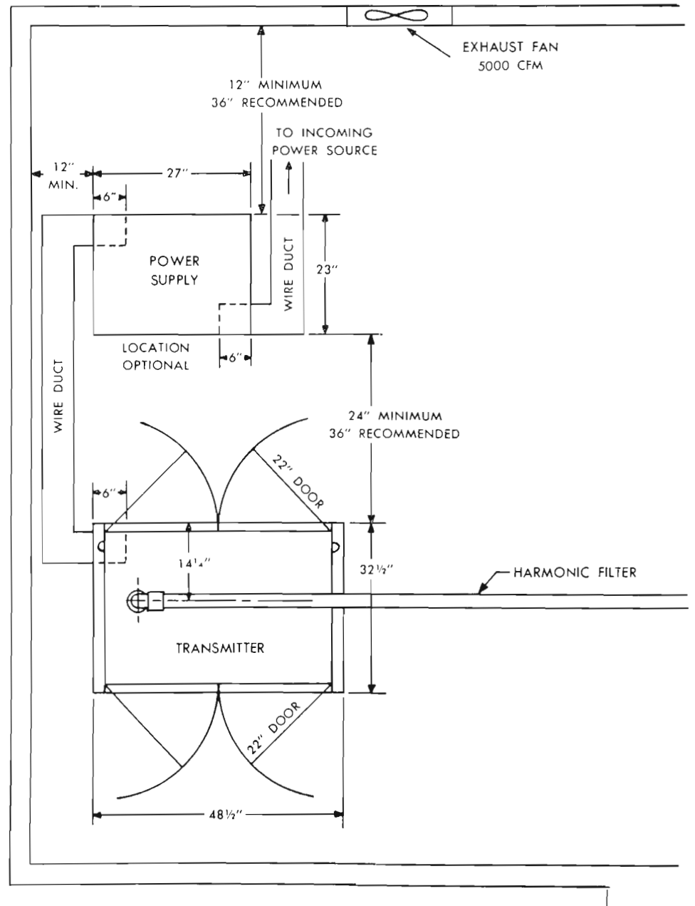
FIG. 8. Floor plan layout for BTF-5 or BTF-10E transmitters.
