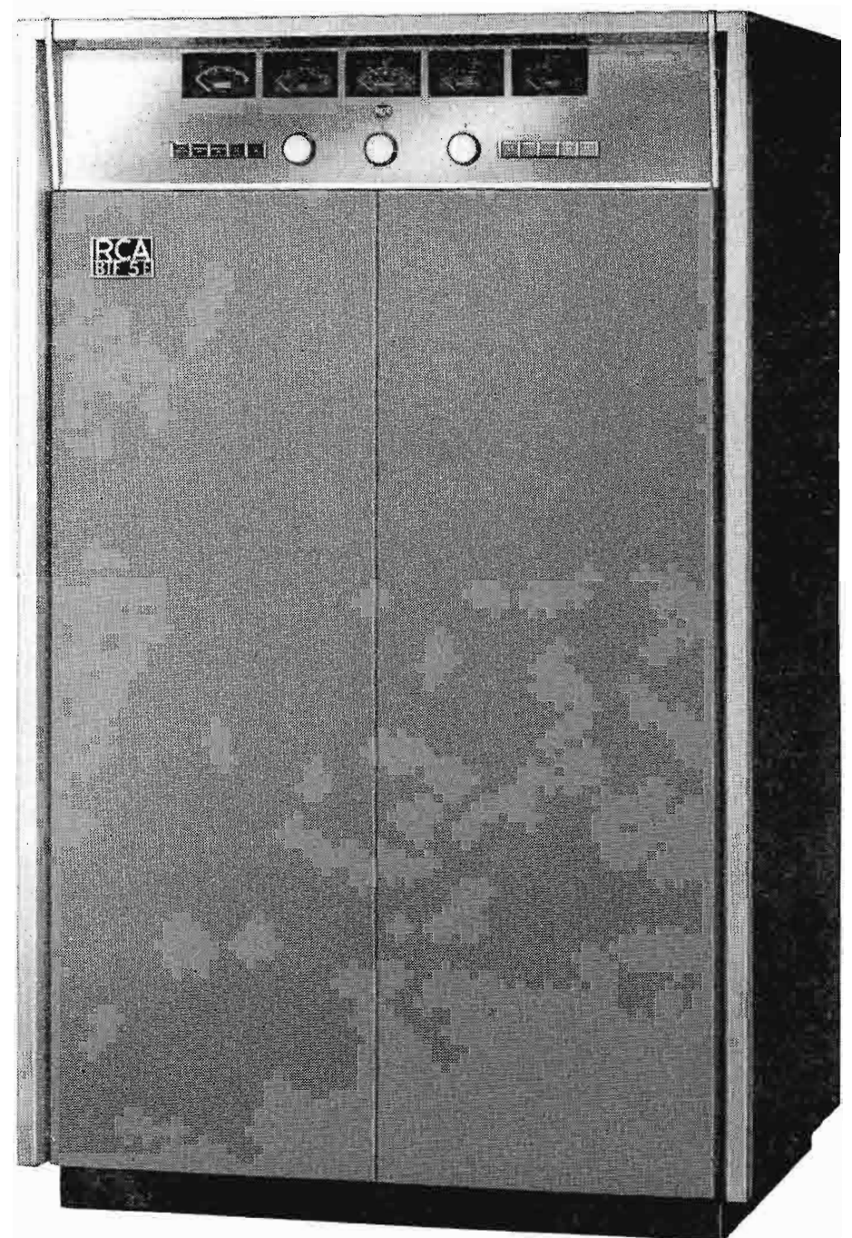
FIG. 10. BTF-5E 5 kW and BTF-10E 10 kW transmitters are in identical cabinets. Circuitry utilizes different output tubes for these transmitters as seen in block diagrams (Fig. 11).
