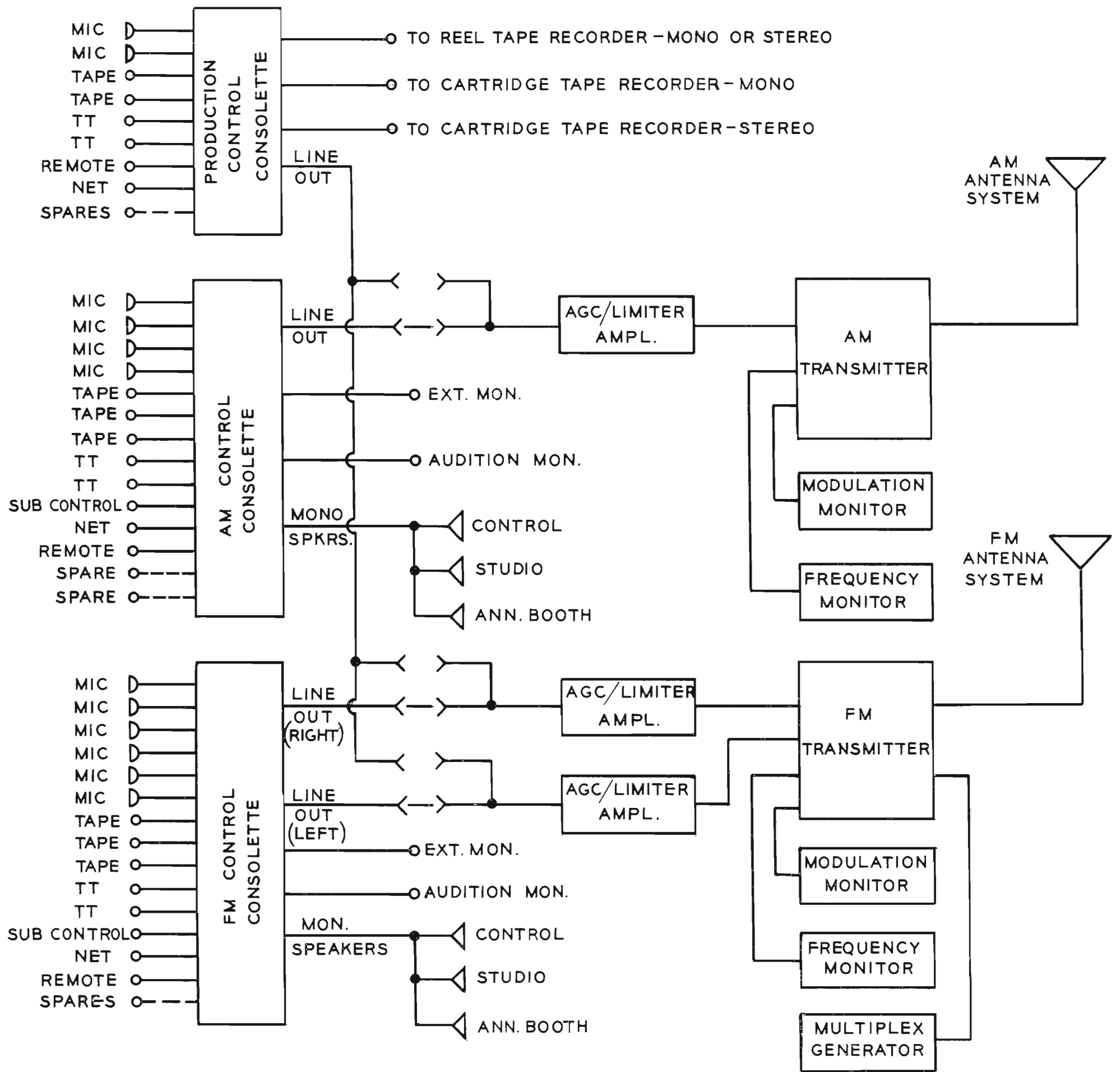
FIG. 13. System diagram of Plan "C" station.
